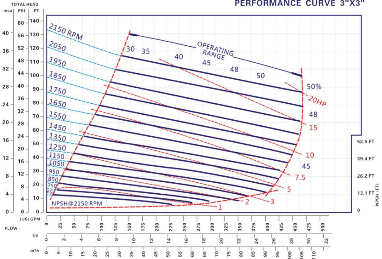
PERFORMANCE CURVE 3"X3"
